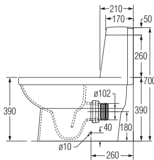
SIDE ELEVATION (180 Connector)
