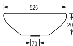
FRONT ELEVATION
