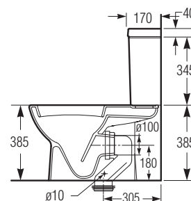
SIDE ELEVATION (305 Connector)
