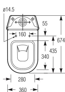
PLAN
