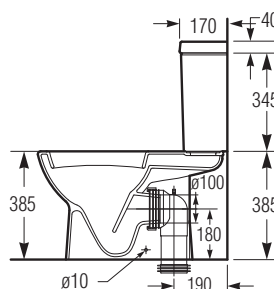
SIDE ELEVATION (190 Connector)
